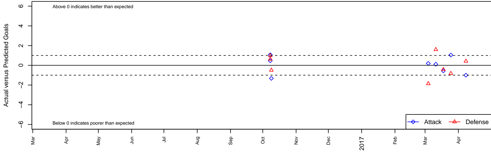
Soccer Xpress Blast G02 Dots are actual minus expected GF (blue circles) and GA (red triangles). Blue line is smoothed change in attack strength. Red is smoothed change in defense strength.
